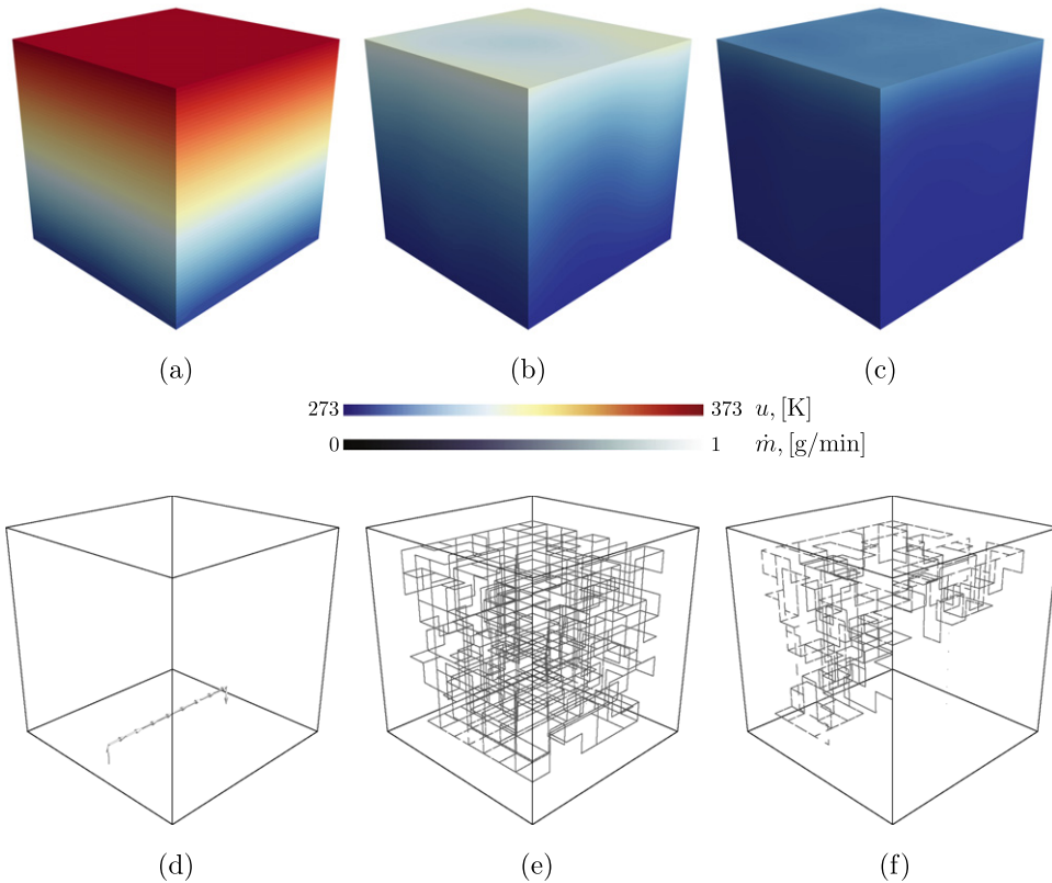
Fig. 7. Selected candidate solutions at generation t = 10000 , marked in the Pareto-optimal front of Fig. 6 with \diamond , \circ , and \square symbols. The upper row shows the temperature field, whereas the figures in the lower row show the corresponding flow field with their corresponding network. Figures (a) and (d) correspond to the individual that minimizes \phi_v , figures (b) and (e) to the individual that minimizes \phi_f and figures (c) and (f) to the one that minimizes \phi_T . Arrows are size-coded according to flow magnitude.
