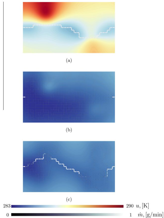
Fig. 11. Selected individuals for the localized heating example obtained with the conventional GA scheme after 5000 generations with a population size |\mathcal{P}| = 1000 . The figures show the temperature field at the surface opposite to where the localized heat sources are applied, and their corresponding networks and flow fields projected on this surface. The temperature range is defined as the minimum and maximum temperature values in the figures. The candidate solutions shown in Figures (a), (b), and (c), minimize objective functions \phi_v , \phi_f , and \phi_T , respectively.
