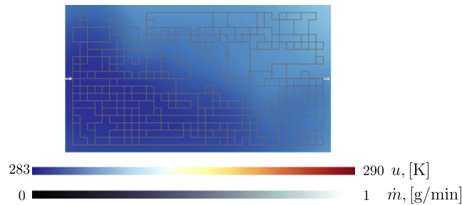
Fig. 13. Candidate solution that minimizes the maximum temperature objective function \phi_T for the knowledge-based GA optimization that started with the evolved population at generation t = 9900 of the 2D optimization. The figure shows the temperature field in the surface located away from the application of the heat sources.
