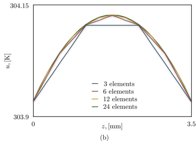
Fig. 3. (a) Temperature profiles obtained at the centerline of the specimen shown in Fig. 2, showing the experimental temperature measurements obtained by infrared imaging, the numerical solutions, and the results of the fin equation. (b) Temperature profile through the thickness obtained numerically at the top of the specimen for meshes with different thickness discretizations.
