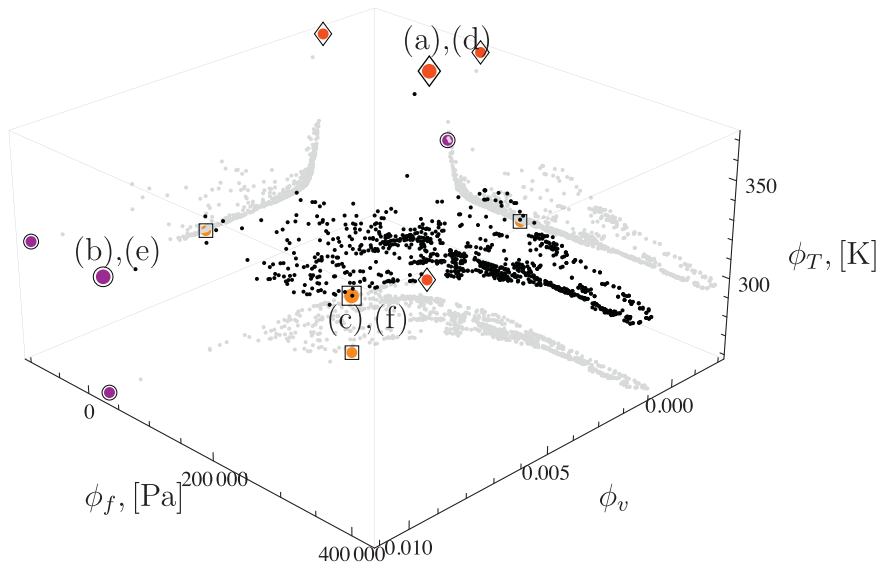
Fig. 6. Pareto-optimal surface at generation t = 10000 for the periodic cell example. Individuals selected for visualization are displayed in Fig. 7 and are labeled in the front and marked with \diamond , \circ , \square symbols.
