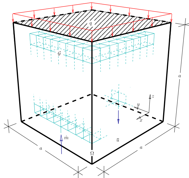
Fig. 5. Schematic of the periodic microvascular cell problem with cubic domain \Omega = a^3 and part of the microvascular network template \mathcal{G} . A single inflow and a single outflow are displayed in the figure with arrows. A uniform heat flux \bar{q} is applied at the top surface, and a temperature \bar{u} is prescribed at the bottom surface. The remaining surfaces have periodic boundary conditions, thus defining a unit cell periodic in the x and y directions.
