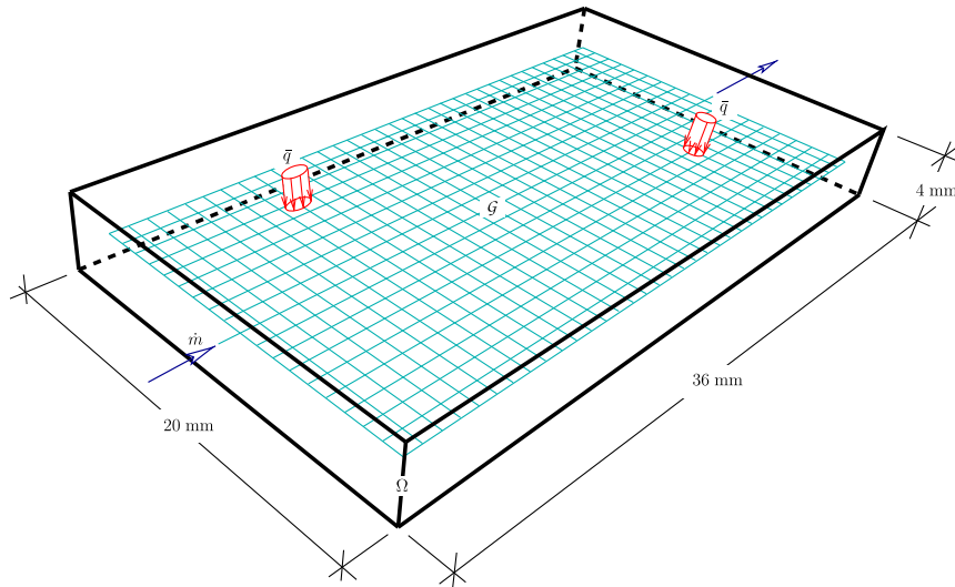
Fig. 8. Schematic of the mathematical model for the localized heating example, showing the domain \Omega and the microvascular network template \mathcal{G} used in the optimization process. Arrows show the location of the inflow and outflow for the flow problem. For the heat boundary value problem, a localized heat flux \bar{q} is applied in two locations over the top surface.
