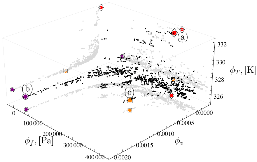
Fig. 10. Pareto-optimal surface at generation t = 5000 for the localized heating example. The optimization is carried out using the 3D finite element model illustrated in Fig. 9. Selected candidate solutions are displayed in Fig. 11 and are labeled in the front and marked with \diamond , \circ , \square symbols.
