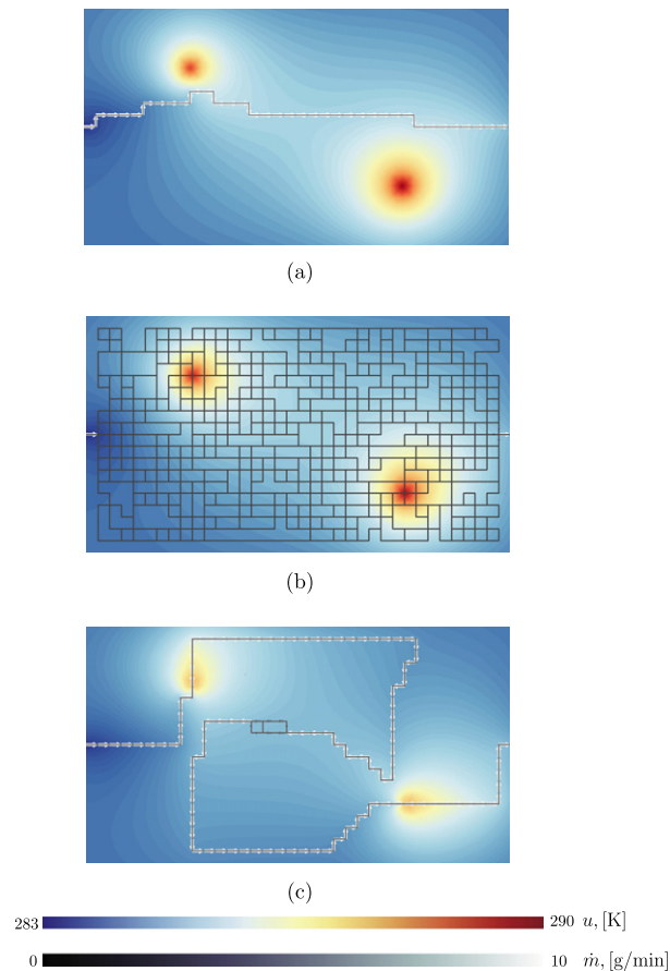
Fig. 12. Figures (a), (b), and (c) show the selected individuals at generation t = 10000 of the 2D optimization, minimizing \phi_v , \phi_f , and \phi_T , respectively.
