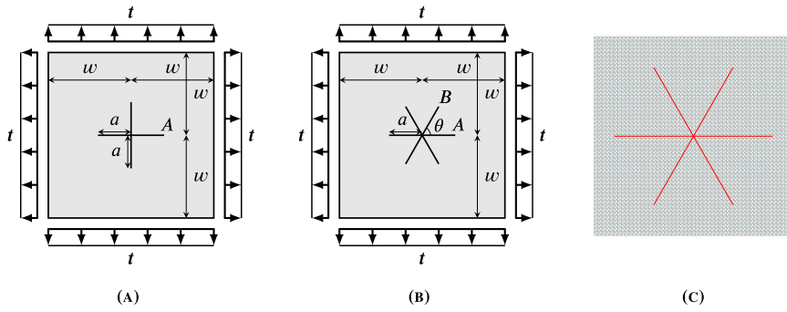
Fig. 13. Cross-shaped (A) and star-shaped ( \theta = \pi/3 ) (B) crack problems, along with (C) the underlying 51 \times 51 triangulated rectangular grid for the a/w = 0.8 configuration of the star-shaped crack problem in (B). The same background mesh is used for the cross-shaped crack problem in (A).
