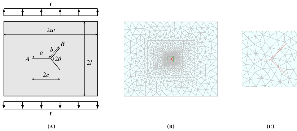
Fig. 11. (A) Symmetric branched crack in a plate subject to uniaxial tension [6] ( l = 16, w = 20, a = b = 1, \theta = \pi/4 ; crack not to scale); (B) underlying unstructured graded mesh used to obtain the first column of results in Table 1 with mesh size h/a = 0.25 and (C) zoomed view around the crack.
