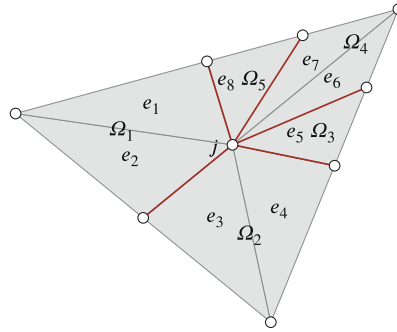
Fig. 6. A triangular domain split by five discontinuities forming a five-fold junction.
