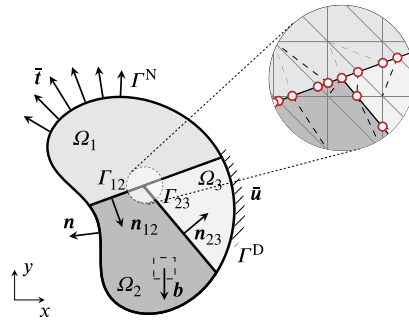
Fig. 1. A two-dimensional domain \Omega composed of disjoint subdomains \Omega_i such that \bar{\Omega} = \cup_i \bar{\Omega}_i and \Gamma_{ij} = \bar{\Omega}_i \cap \bar{\Omega}_j ( i \neq j ). Dirichlet and Neumann boundary conditions are prescribed on \Gamma_i^D and \Gamma_i^N , respectively. The zoomed-in inset shows the unfitted mesh intersected by discontinuity segments, forming a triple junction. The red circles indicate new nodes with enriched degrees of freedom. The background mesh is depicted with thin solid lines, while the integration elements in the elements cut by the discontinuities are shown with dashed lines.
